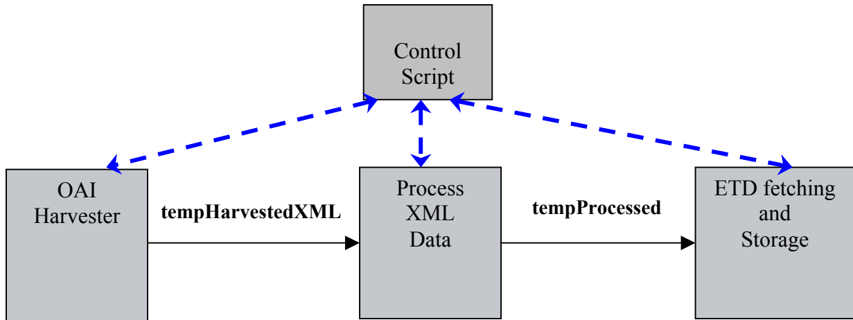
Figure 2. System Architecture
